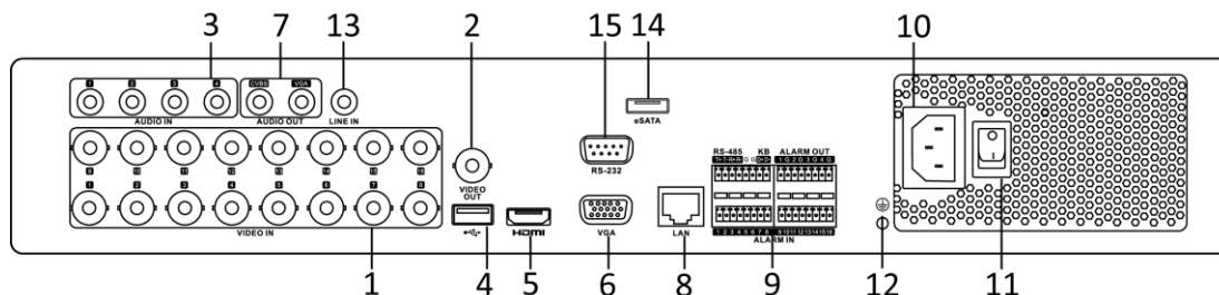
Figure 1. 12 DS-7300HQHI-SH and DS-7300HGHI-SH
