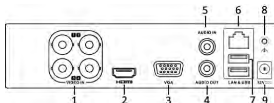
Figure 1. 9 DS-7100HGHI-SH and DS-7100HQHI-SH
